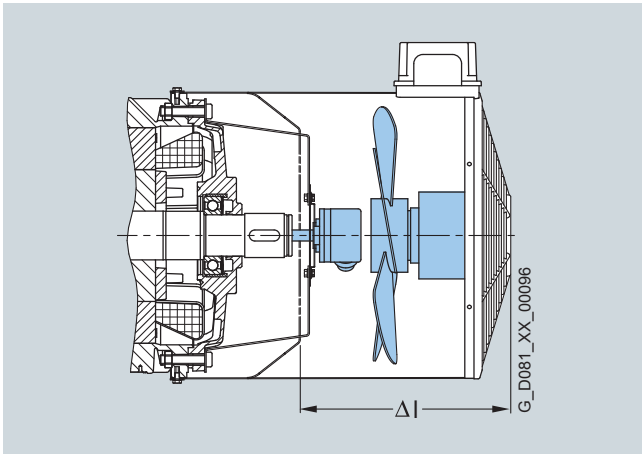
Motor with encoder and separated driven fan
