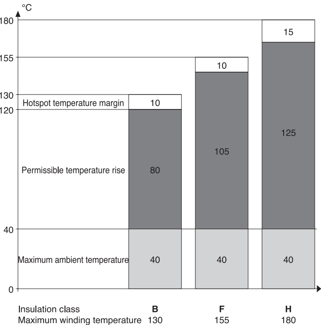
Saftey margins per insulation class
