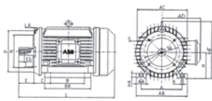
terminal box side-mounted IM B34 (on request)
